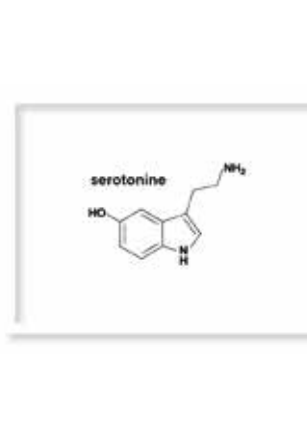
Serotonine
